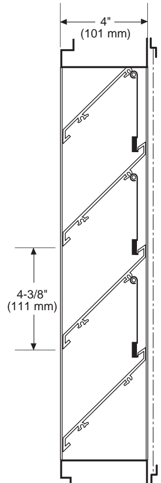
CHANNEL FRAME
