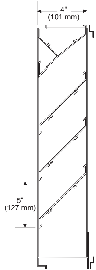
Channel Frame
