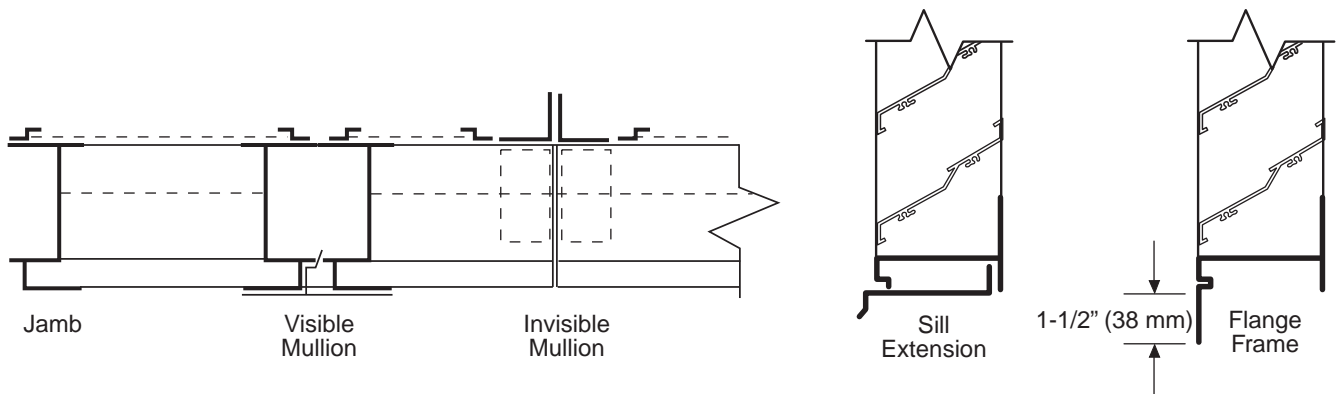
Channel Frame
