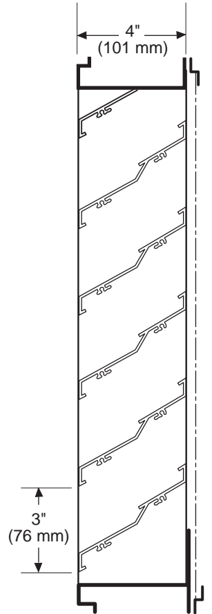
Channel Frame
