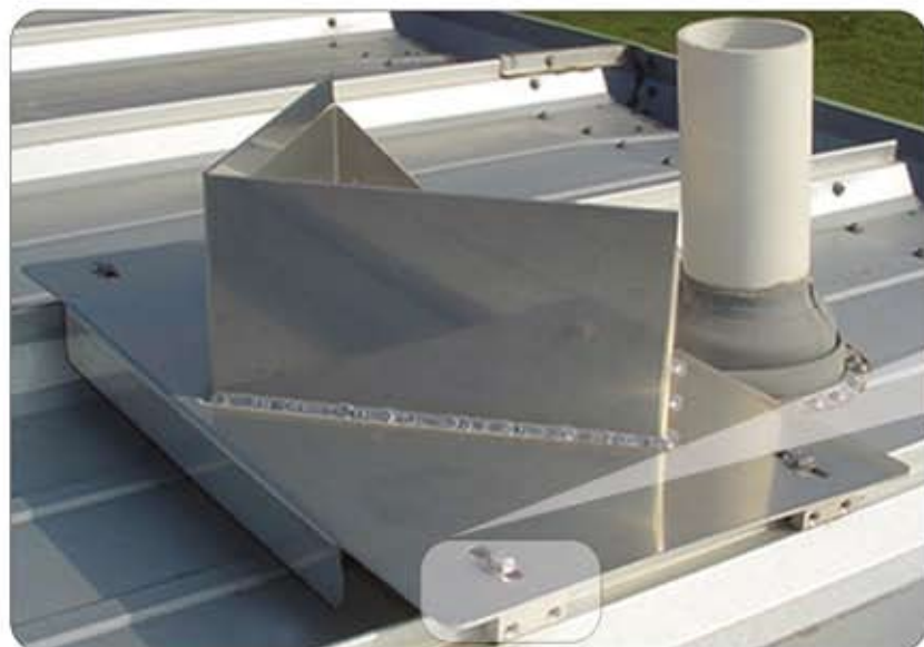
Leaking Roof
