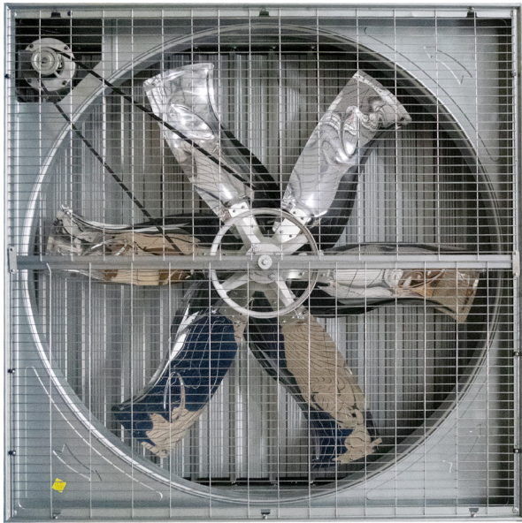
30" Belt drive exhaust fan in cabinet
